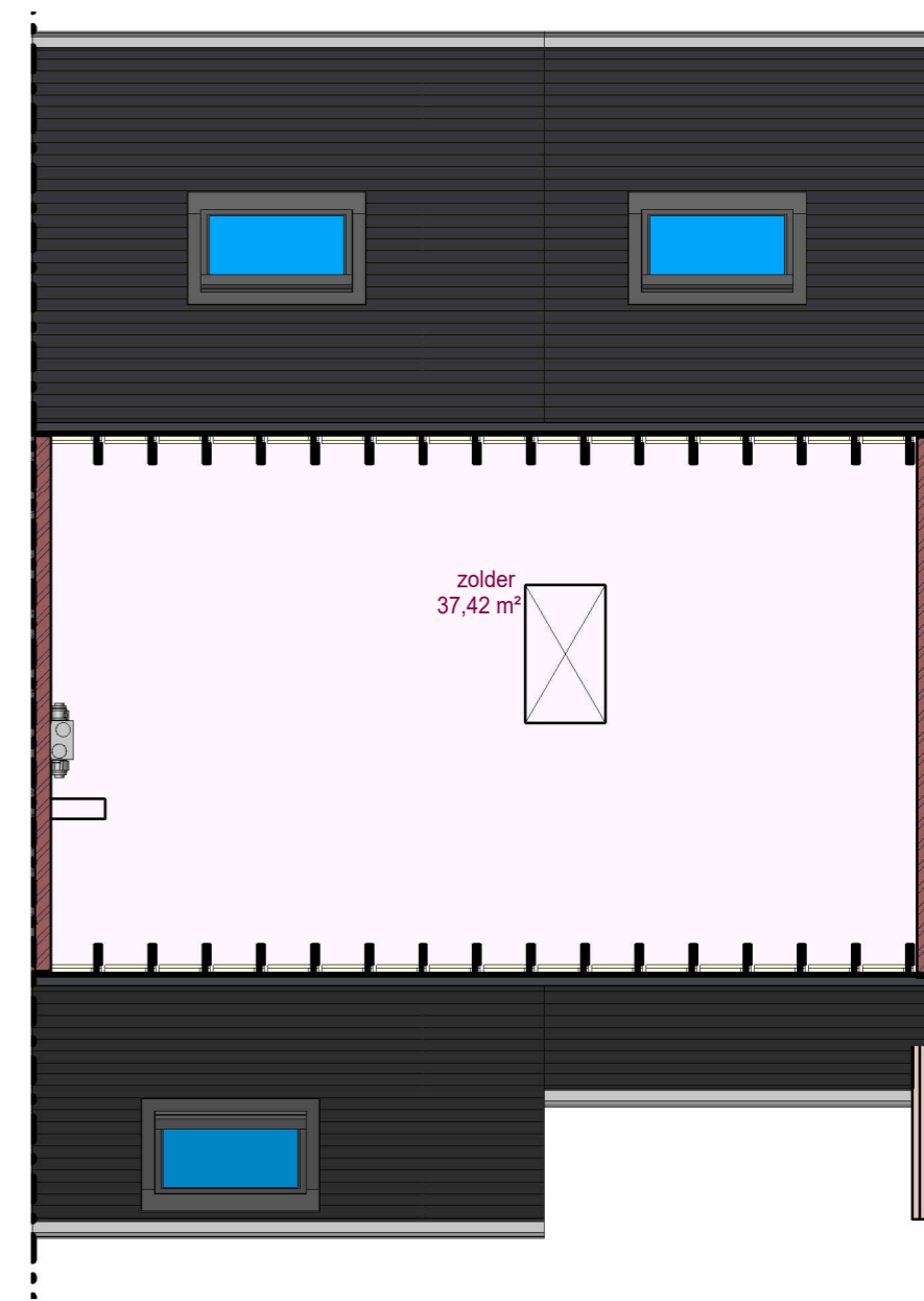
3 Zolder verdieping 178 LL 1 : 70
